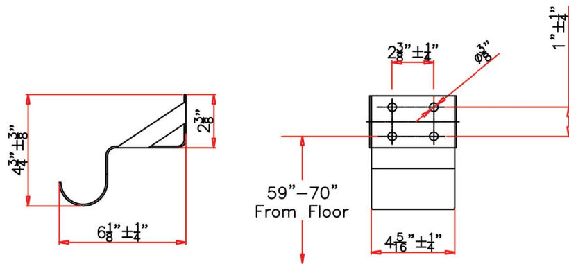
SUPPORT BRACKET
